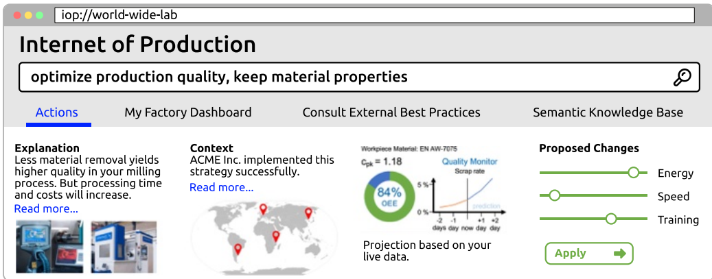
Fig. 1. A mockup of a search engine for production queries leveraging the (global) knowledge base processed by intelligent agents to optimize production processes, as envisioned by the IoP.
