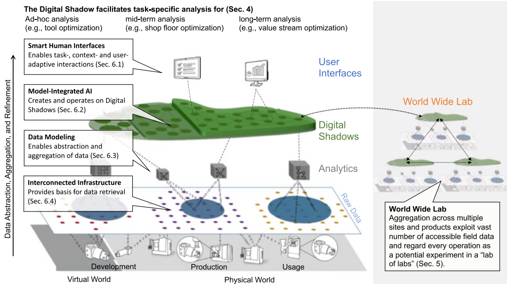
Fig. 2. In the IoP, task-adaptive Digital Shadows build on interconnected infrastructure, data modeling, and model-integrated AI to provide smart interfaces that make the right data actionable at the right time during development, production, and usage. Integration across different production facilities and locations leads to the WWL.
